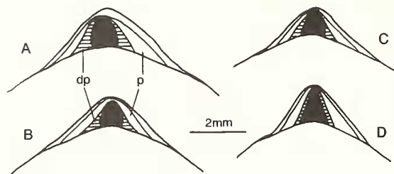
TEXT-FIG. 6. Pedicle opening and related structures from juvenile (D) to adult (A) stages. dp = deltoidal plate; p = palintrope. A, sample C-E, PUM92054. B, sample L17, PUM92055. C, sample C-C, PUM92056. D, sample C-D, PUM92057. Specimens of A and B uniplicate, whereas in the latter two, the sulcus has not developed and sinal plication cannot be defined.
